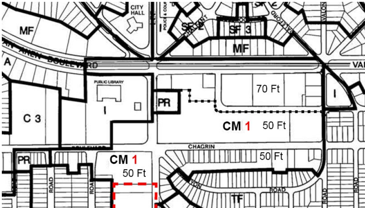
Figure 1234.08-B Maximum Height Requirements Van Aken/Warrensville Area CM-1 Commercial Mixed Use District
